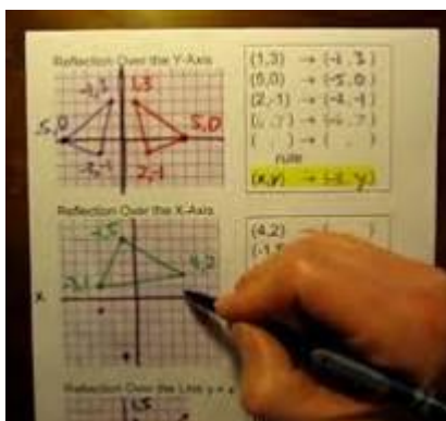
Figure Coordinate Rules For Reflections on a Graph.MOV
